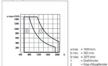
RWA 105 NT Syncro
